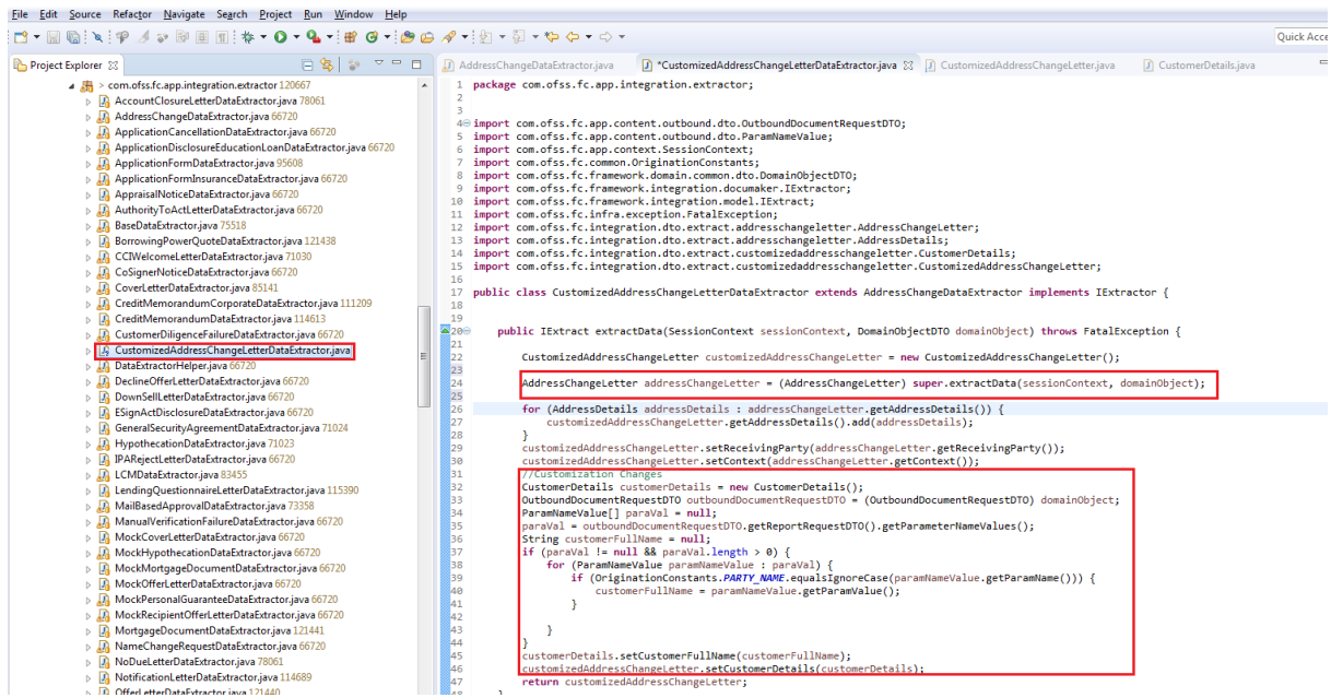
Figure 18–8 Customized AddressChangeLetterDataExtractor
