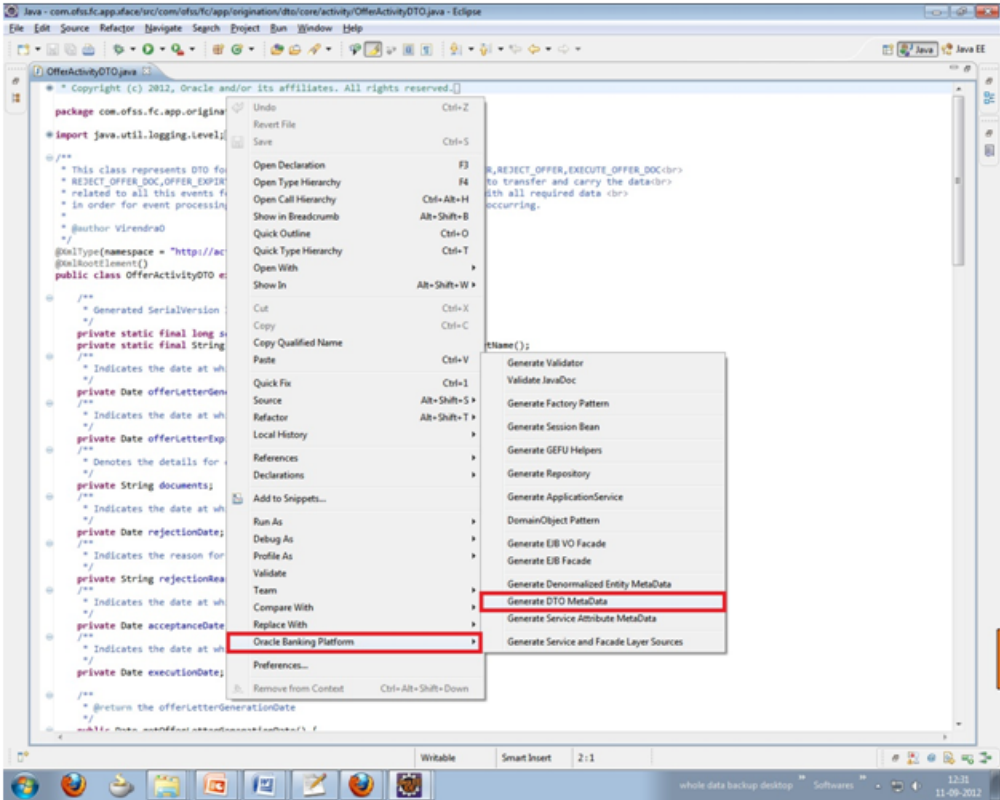
Figure 10-5 Metadata Generation
