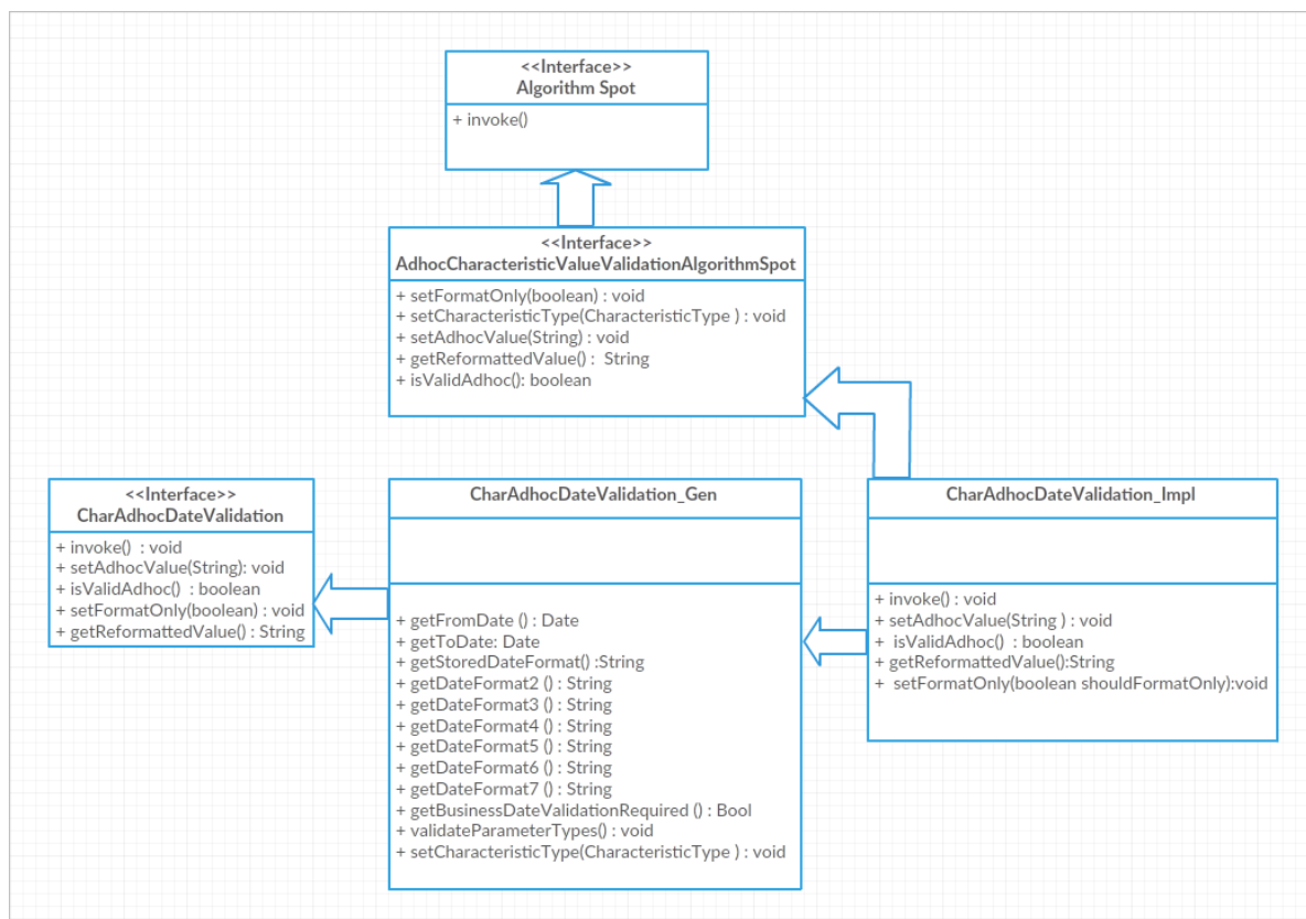
Figure 19–4 Example: Data Validation Algorithm Component
