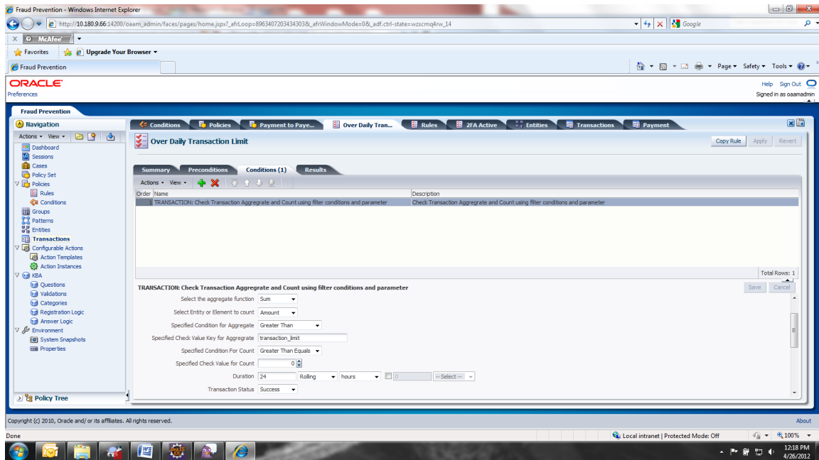
Figure 12–10 Add or Modify Fraud Rules in OAAM - Conditions Tab
