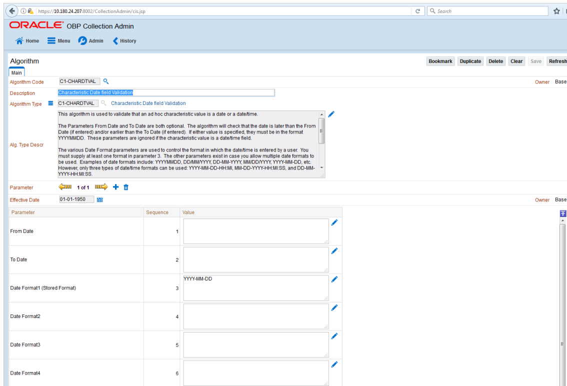
Figure 19–13 Attach Algorithm
