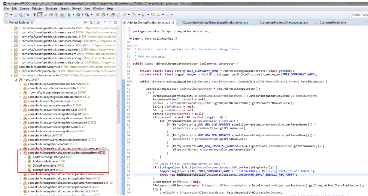
Figure 18–3 JAXB Classes
