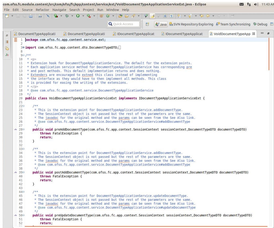
Figure 4–3 Default Application Service Extension
